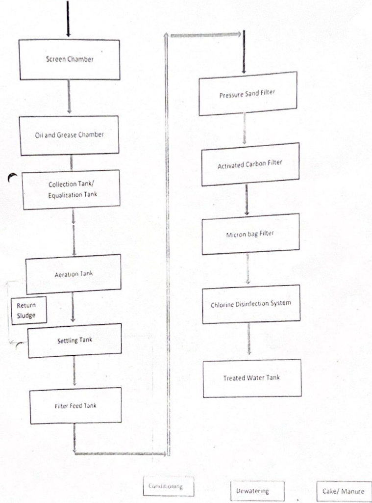
Flow Diagram Raw Sewage Water
